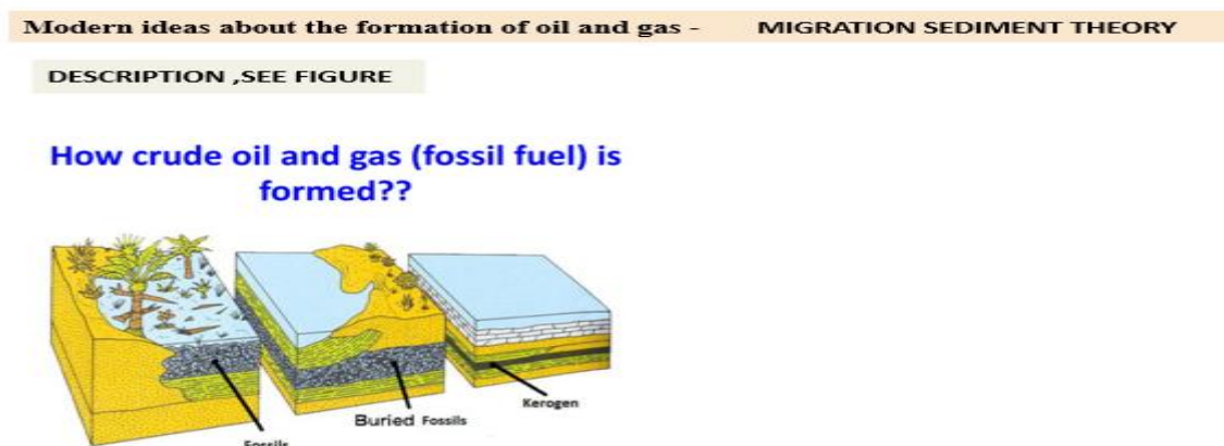
Figure 2 Modern ideas about the formation of oil and gas
